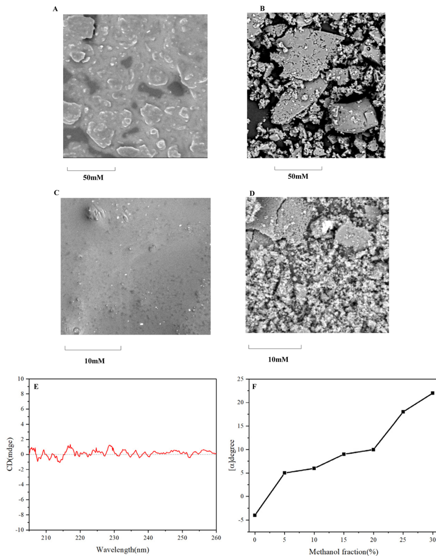
Fig. 7 (A) and (C) SEM picture of polymers 3 and 4. (B) and (D) SEM picture of polymers 3 and 4. (E) CD spectra of polymer 3 (0.02 mg in methanol). (F) Aggregation-induced polarization (AIP) of polymer 3 in THF and methanol mixture.
