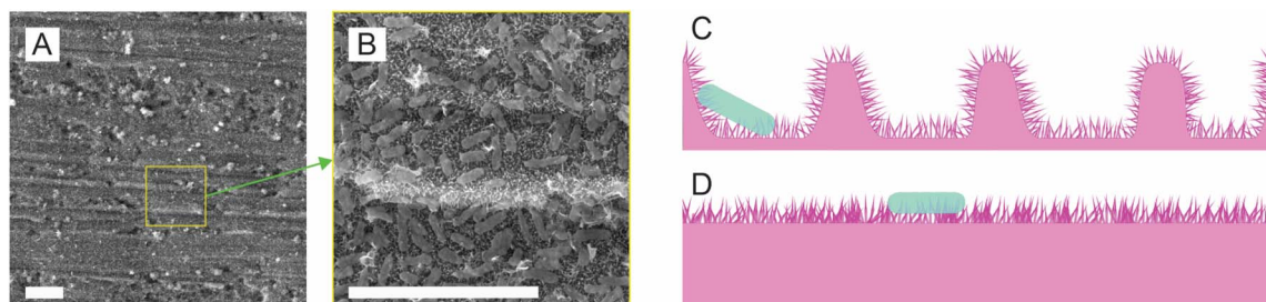
Fig. 8 (A) SEM image at 2k\times magnification of the 1.44 \mu\text{mRa} surface with P. aeruginosa bacteria on it. Scratch marks from the sanding surface can be seen on the surface (horizontal lines). (B) The same surface at 10k\times magnification. The bacteria can be observed in the valley area of the scratch marks. Scale bar 10 \mu\text{m} . (C) Nanowires on the roughened substrate. The uneven topography of the roughened substrate leads to nanowires protruding from the surface in multiple directions and (D) the pictorial illustration (not to scale) of the nanowires on the smooth substrate.
