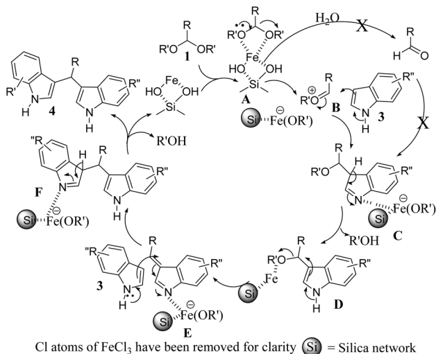
Fig. 2 Proposed reaction mechanism of the \text{FeCl}_3/\text{SiO}_2 -catalyzed bis-indolylmethane synthesis.
