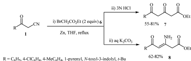
Scheme 3 Synthesis of 3,5-dioxopentanoates 7 (3,5-diketo esters) and 3-amino-5-oxopent-3-enoates 8 .
