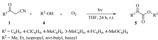
Scheme 2 Reactions of β-ketonitriles and alcohols for constructing α-ketoesters 5 .
