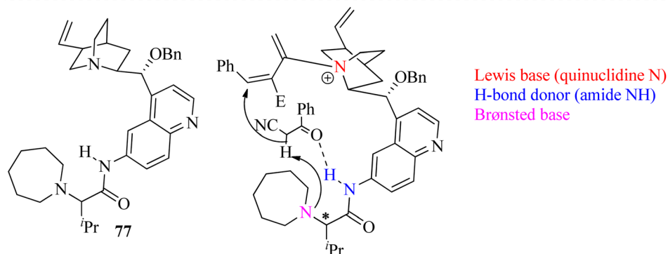
Scheme 30 Synthesis of 4H-pyran derivatives 78 by using 6'-deoxy-6'-(L)-N,N-(2,2'-oxydiethyl)-valine amidoquinine 77 as a catalyst.
