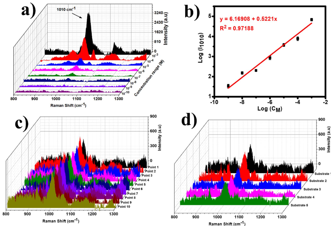
Fig. 7 (a) SERS spectra of urea ( 10^{-3} M to 10^{-10} M) on ZIF-8/Ag. (b) The plot of the log of SERS intensity at 1010 \text{ cm}^{-1} against urea concentration. (c) Uniformity and (d) reproducibility of SERS sensors for urea on ZIF-8/Ag substrate.
