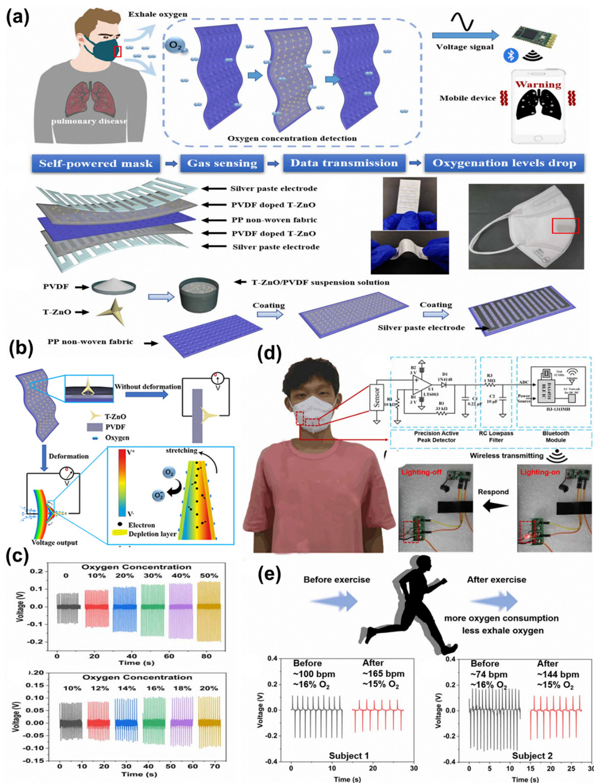
Fig. 15 (a) Schematic of the self-powered exhalation-oxygen-sensing mask and its fabrication process. (b) Working mechanism of the piezoelectric gas sensor under deformation. (c) Sensor response to different oxygen concentrations. (d) Practical application of the mask with wireless data transmission and LED response. (e) Sensor validation before and after exercise for two subjects. Reproduced with permission, 63 Copyright © 2022 IOP Publishing Ltd.
