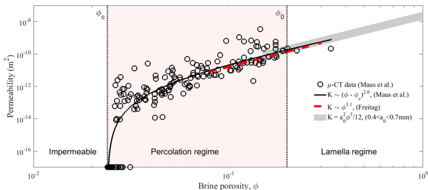
Fig. 1 Vertical permeability simulations versus brine porosity with best columnar ice fit from Maus et al. 21 compared to the relationship obtained by Freitag 24 for young ice (red curve), and the lamella model at high porosity (eqn (5)) for a typical range in sea ice plate spacing). The regime boundary for \phi_0 described in the text is chosen tentatively.
