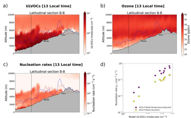
Fig. 7 (a) Modelled ULVOCs concentrations (molecules per \text{cm}^3 per s), (b) ozone concentrations along the latitudinal profile B–B (ppb), and (c) total nucleation rate (particles per \text{cm}^3 per s), of the Khumbu valley at 13 local time. The effect of the temperature correction on the nucleation rate is presented as a scatterplot, (d).
