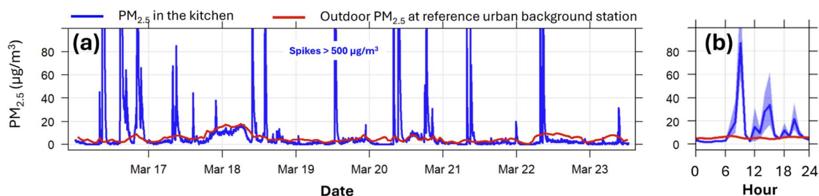
Fig. 8 Indoor and outdoor \text{PM}_{2.5} concentrations in one of the sampled kitchens during March 2024 over a week in \mu\text{g m}^{-3} . (a) Indoor PM levels closely follow outdoor levels indicating the contribution of outdoor generated pollution indoors with clear events ( i.e. cooking) elevating indoor levels above outdoor background. (b) A clear diurnal profile can be noticed for indoor sources driven by behavioural patterns of the occupants (active emissions). Calculated mean with 95% confidence interval in the mean.
