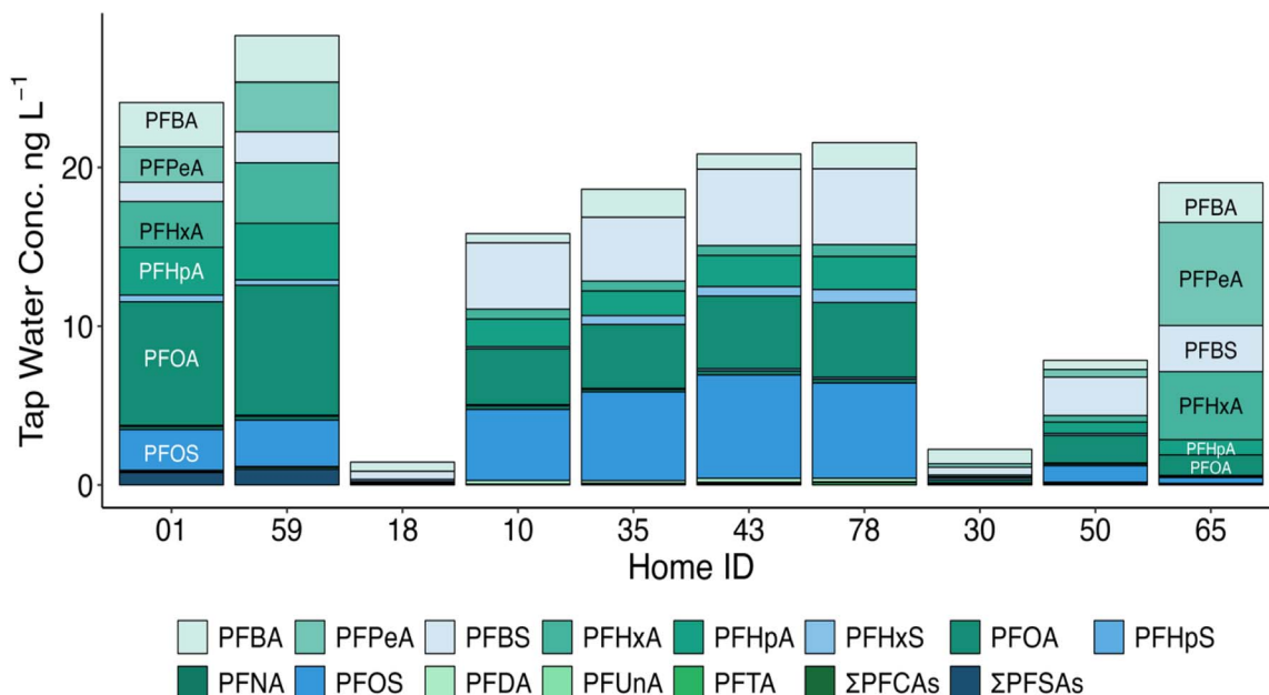
Fig. 2 PFAA profiles and concentrations in kitchen tap water samples. Compounds with DF > 50% are shown while those with DF < 50% were summed into their respective subclass (i.e., \Sigma PFCA or \Sigma PFSA). All carboxylic acids (PFCA) are in shades of green and the sulfonic acids (PFSA) are in shades of blue. Each bar is plotted such that PFBA is on top, followed by PFPeA and PFBS, with \Sigma PFCA and \Sigma PFSA last. Concentrations are mean field blank subtracted and corrected for recoveries.
