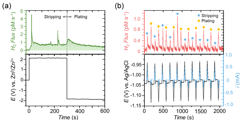
Fig. 5 (a) H 2 flux profile and E - t profile for galvanostatic stripping and plating of Zn at 1 mA cm -2 in 2 M ZnSO 4 on a Zn WE. (b) H 2 flux profile and both E - t and i - t profiles for cyclic voltammetric stripping and plating of Zn in 10 mM ZnSO 4 on a Zn WE. The potential window was ±100 mV from the OCP.
