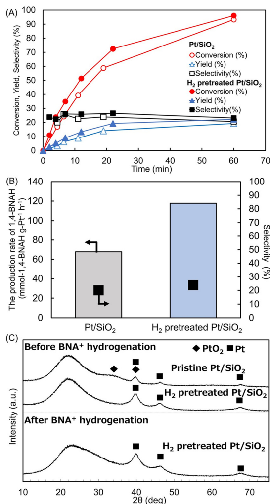
Fig. 5 (A) Time course of \text{BNA}^+ hydrogenation using Pt/SiO 2 catalyst and \text{H}_2 -pretreated Pt/SiO 2 catalyst. The reaction conditions: \text{BNA}^+ (1.5 mmol L -1 ) in 20 mL of 0.1 mol L -1 Tris-HCl buffer (pH 8.8) with a 4 wt% Pt/SiO 2 catalyst (5 mg) at 20 °C under 1 atm \text{H}_2 . (B) Comparison of the 1,4-BNAH production rates. (C) XRD patterns of the 4 wt% Pt/SiO 2 catalyst comparing of pristine, without \text{H}_2 pretreated, and \text{H}_2 pretreated samples at before (upper) and after (lower) \text{BNA}^+ hydrogenation.
