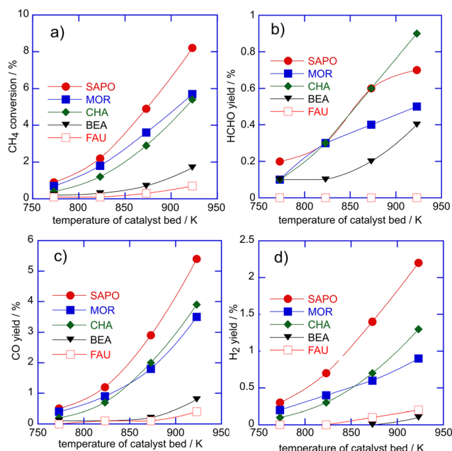
Fig. 2 Methane oxidation with \text{O}_2 over Cu catalysts supported on different zeolites. a) \text{CH}_4 conversion, b) yield of HCHO, c) yield of CO and d) yield of \text{H}_2 .
