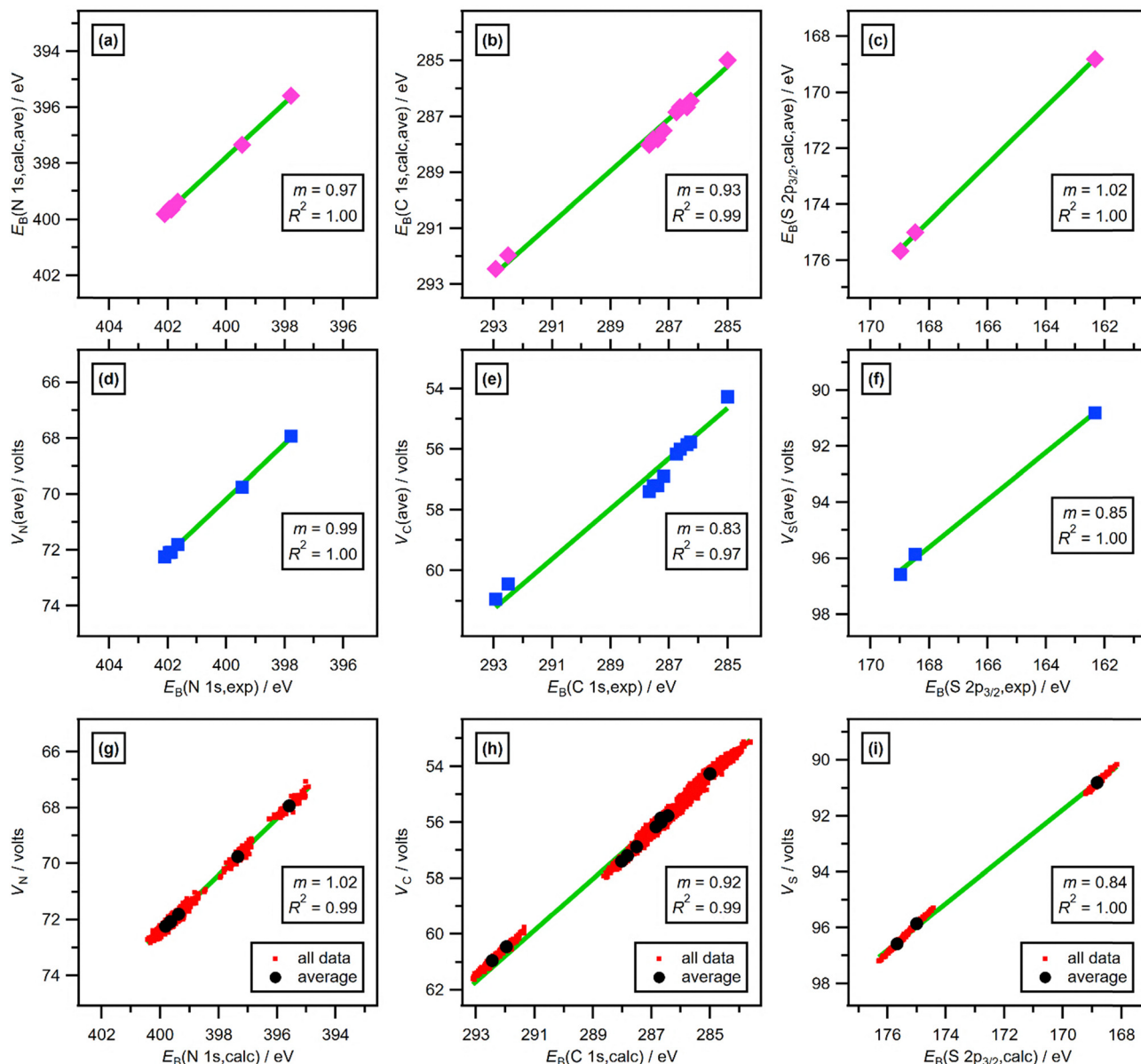
Fig. 2 E_B(\text{core}, \text{calc}, \text{ave}) plotted against E_B(\text{core}, \text{exp}) for [\text{C}_8\text{C}_1\text{Im}]\text{Cl} , [\text{C}_8\text{C}_1\text{Im}][\text{SCN}] , [\text{C}_8\text{C}_1\text{Im}][\text{TfO}] and [\text{C}_8\text{C}_1\text{Im}][\text{NTf}_2] : (a) N 1s (data for both cations and anions), (b) C 1s (data for both cations and anions), (c) S 2p 3/2 (data for anions). V_N(\text{ave}) plotted against E_B(\text{core}, \text{exp}) for [\text{C}_8\text{C}_1\text{Im}]\text{Cl} , [\text{C}_8\text{C}_1\text{Im}][\text{SCN}] , [\text{C}_8\text{C}_1\text{Im}][\text{TfO}] and [\text{C}_8\text{C}_1\text{Im}][\text{NTf}_2] : (d) N 1s (data for both cations and anions), (e) C 1s (data for both cations and anions), (f) S 2p 3/2 (data for anions). V_N (all individual data points and average) plotted against E_B(\text{core}, \text{calc}) for [\text{C}_8\text{C}_1\text{Im}]\text{Cl} , [\text{C}_8\text{C}_1\text{Im}][\text{SCN}] , [\text{C}_8\text{C}_1\text{Im}][\text{TfO}] and [\text{C}_8\text{C}_1\text{Im}][\text{NTf}_2] : (g) N 1s (data for both cations and anions), (h) C 1s (data for both cations and anions), (i) S 2p 3/2 (data for anions). R^2 = coefficient of determination and m = gradient. Full equations for the correlations are given in SI, Table S12.
