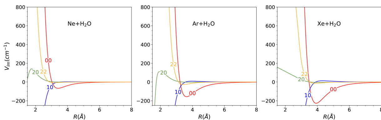
Fig. 8 Partial wave expansion coefficients of the PES ( v_{l,m} ) as a function of R for \text{Ne} + \text{H}_2\text{O} (left panel), \text{Ar} + \text{H}_2\text{O} (middle panel) and \text{Xe} + \text{H}_2\text{O} (right panel). The partial wave numbers are indicated in each curve, and only the four first partial waves are presented.
