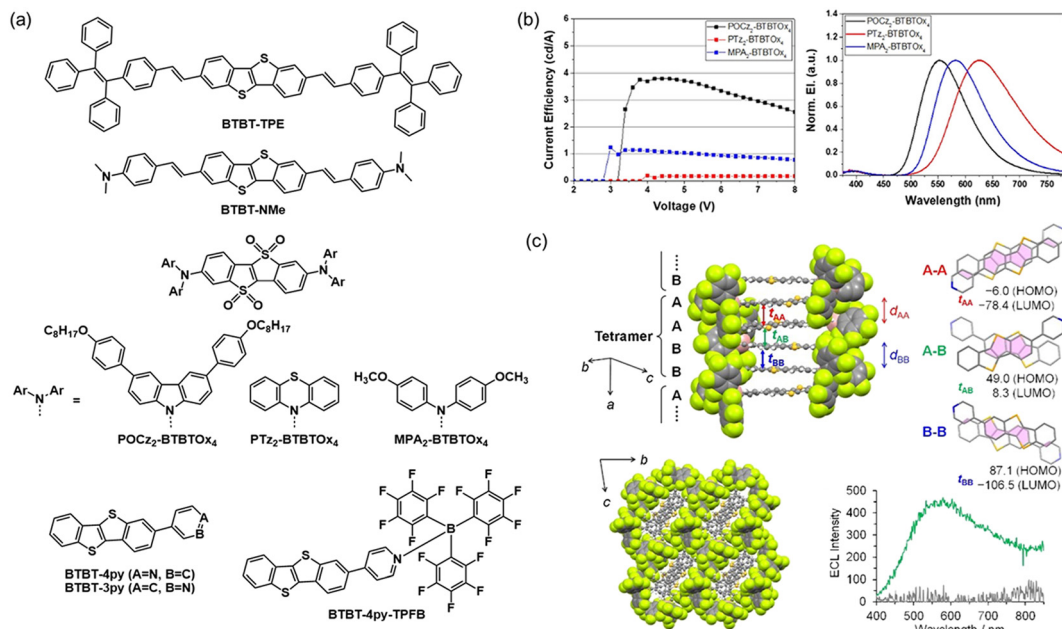
Fig. 12 (a) Structures of BTBT-based luminescent molecules. (b) The current efficiency and electroluminescence spectra of OLEDs using POCz 2 -BTBT x 4, PTz 2 -BTBT x 4 and MPA 2 -BTBT x 4 as emitting layers. Reprinted with permission from ref. 104. Copyright 2025, The Royal Society of Chemistry. (c) Crystal structures of BTBT-4py-TPFB with transfer integral values and electrochemiluminescence from the crystalline film of BTBT-4py-TPFB with a co-reactant in PBS aqueous solutions. Reprinted with permission from ref. 97. Copyright 2023, Wiley-VCH.
