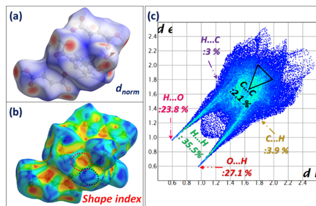
Fig. 18 Hirshfeld surface analysis in d_{\text{norm}} (a) and shape index modes (b) and the calculated fingerprint plots (c) of m -xylylenediamine/fumaric acid-trihydrate salt (VI).
