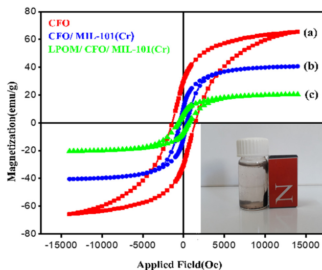
Fig. 7 Magnetization curves of (a) CFO, (b) CFO/MIL-101(Cr) and (c) the LPOM@MIL-101(Cr)/CFO nanocomposite.
