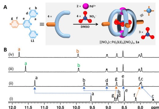
Fig. 1 (A) Schematic for the stoichiometry-controlled synthesis of a building block cage, 1a ; (B) 1 H NMR spectra of (i) ligand L1 , (ii) isolated NO 3 -1.3NO 3 , 1a , and (iii)/(iv) halide-encapsulated cages obtained upon addition of 1 equiv. of TBACl/TBABr to 1a .
