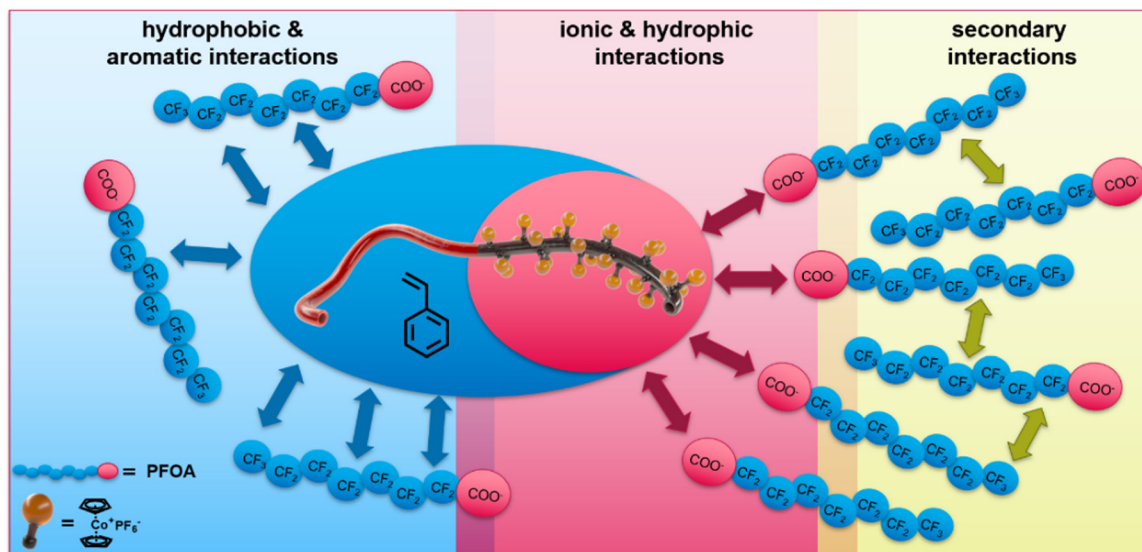
Fig. 1 Possible interaction between the synthesized cobaltocenium-containing block copolymer polystyrene- b -(polycobaltoceniummethyl tert -butylaminoethyl methacrylate-co-polymethyl methacrylate) (PS- b -(PCoEtBAEMA-co-PMMA)) and perfluorooctyl acid (PFOA) and resulting secondary interaction effects.
