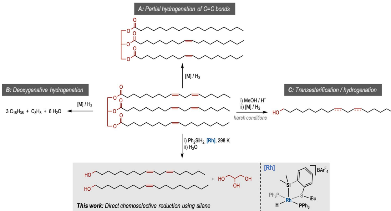
Fig. 1 Different pathways for the reduction of plant oils and the structure of the [Rh(Si S Bu)] complex used in this study.
