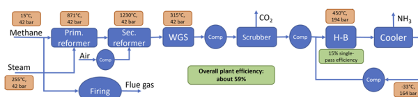
Fig. 2 Simplified process flow diagram of the conventional ammonia synthesis process. "WGS" is the water gas shift reactor, "H–B" the Haber–Bosch reactor and "Comp" are compressors. The process has two main sources of CO 2 emissions: process CO 2 from the scrubber, and CO 2 from the flue gas stream of the firing. The former is associated with lower capture costs as the CO 2 is at high partial pressure, it is already separated from the process gas stream during normal operation. Capturing and storing CO 2 from the flue gas however will incur higher costs, as the partial pressure of the CO 2 is lower and an additional carbon capture plant is required.
