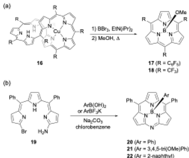
Scheme 4 (a) Metathesis-like ring splitting of heptaphyrin 16 , and (b) boron-templated synthesis of submonoazaporphyrins.
