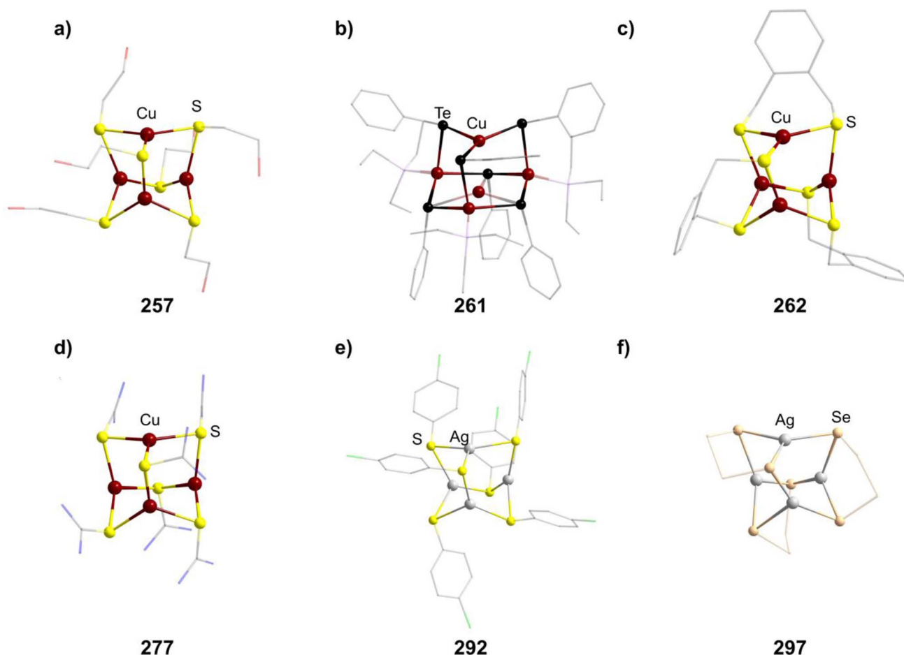
Fig. 9 Examples of adamantane-type compounds with group 11 in the Q-position and group 16 atoms in the E-position: [\text{tBu}_4\text{N}]_2[\text{Cu}_4\{o\text{-(SCH}_2\text{CH}_2\text{OH})_6\}] ( 257 , top left (a)), [\text{Et}_3\text{PPh}][\mu_3\text{-Cu}(\text{CuPEt}_3)_3\text{Cu}(\text{TePh})_6] ( 261 , top center (b)), [\text{Ph}_4\text{P}]_2[\text{Cu}_4\{o\text{-(SCH}_2)_2\text{C}_6\text{H}_4\}_3] ( 262 , top right (c)), [\text{Cu}_4\{\text{SC}(\text{NH}_2)_2\}_6](\text{SO}_4)_2 ( 277 , bottom left (d)), [\text{Et}_4\text{N}]_2[\text{Ag}_4(\text{SC}_6\text{H}_4\text{-}p\text{-Cl})_6] ( 292 , bottom center (e)) and [\text{tPr}_4\text{N}]_2[\text{Ag}_4(\text{Se}_4)_3] ( 297 , bottom right (f)). Hydrogen atoms and counterions, if present, are omitted for clarity.
