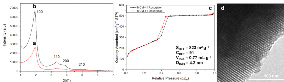
Fig. 5 XRD patterns of (a) as-synthesized MCM-41 and (b) surfactant extracted MCM-41, (c) \text{N}_2 sorption isotherm at 77 K and (d) TEM image of surfactant extracted MCM-41.
