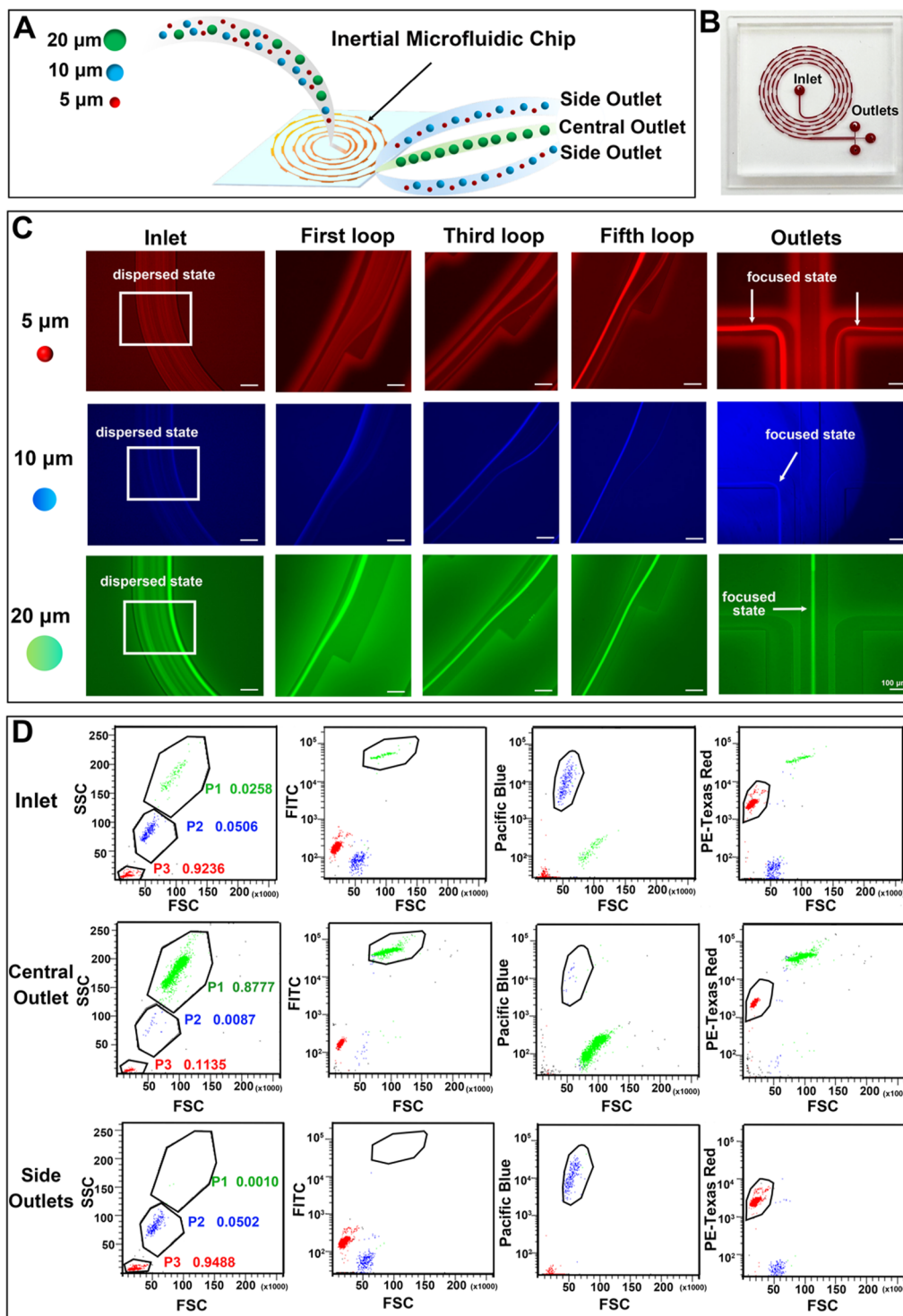
Fig. 4 Separation effect of fluorescent microspheres by inertial microfluidic chip. Separation diagram of mixture of three types of micro-particles with diameter of 5 \mu\text{m} , 10 \mu\text{m} and 20 \mu\text{m} (A); photograph of inertial microfluidic chip with inlet, spiral channel, and outlets (B); fluorescent pictures of particles' trajectories in outlet, first loop, third loop, fifth loop and outlets (C); comparison of fluorescent intensity and proportion of particles in collected liquid sample from inlet, central outlet and both side outlets (D).
