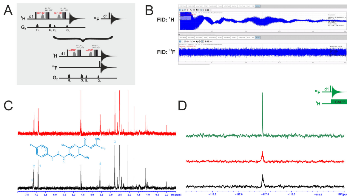
Fig. 3 A: Pulse sequences for the single-receive experiments and the multi-receive experiment, respectively. B: FIDs of the multi-detected experiment with a shorter acquisition time for 19 F. C: The individually recorded 1 H-1D spectrum in red and the 1 H-1D from the multi-detected experiment in black. Relevant signals of the compound are assigned. D: 19 F-1D spectrum from the multi-detected experiment in black, the single recorded spectrum in red and the 19 F-1D with 1 H decoupling in green. The experiments were recorded with 512 scans at a field strength of 600 MHz.
