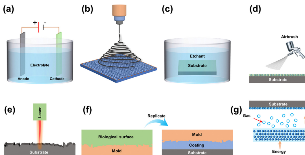
Fig. 9 Schematic representation of a common manufacturing method for bio-inspired microtextured surfaces, including (a) electroplating, (b) electrospinning, (c) chemical etching, (d) spray coating, (e) laser processing, (f) template method, and (g) CVD.
