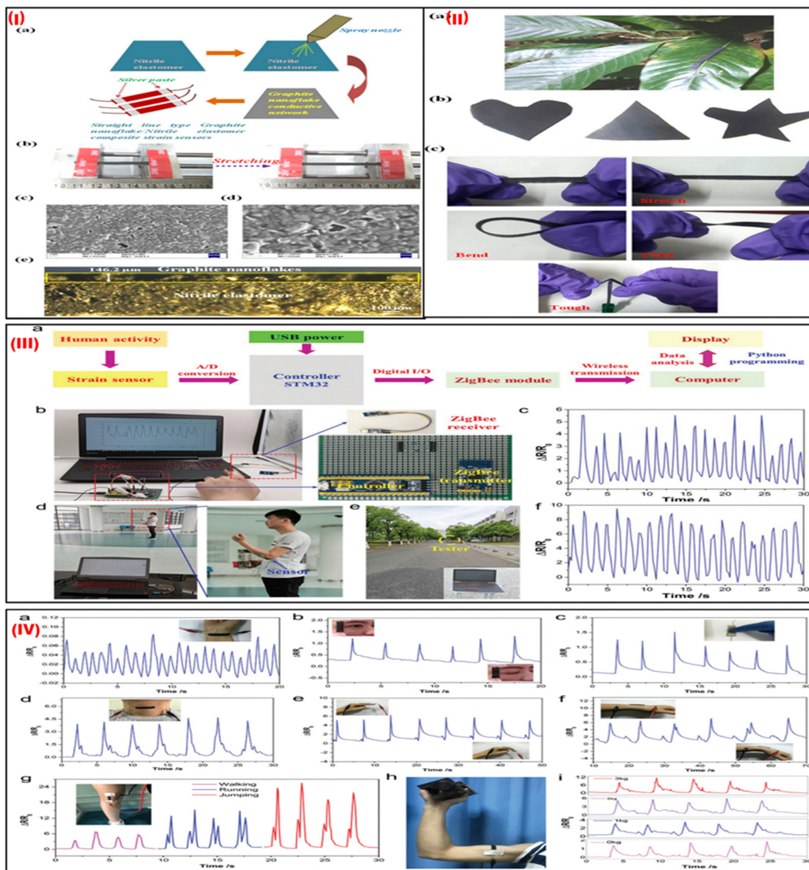
Fig. 5 (I) (a) The manufacturing procedure for strain sensors made of an ultrasensitive graphite nanoflake/nitrite elastomer composite. (b) The tensile strains revealed the good stretchability of the strain sensor. (c) An SEM picture of the conductive network made up of graphite nanoflakes. (d) A magnified SEM picture of (c). (e) A cross-sectional optical image of the graphite nanoflake/nitrite elastomer nanocomposite strain sensors. (II) (a) Strain sensors are robust and resilient, and lightweight and can be placed on leaves. (b) Various shapes of a graphite nanoflake/nitrite elastomer nanocomposite. (c) Graphite nanoflake/nitrite elastomer nanocomposite strain sensors are tough and can be stretched, bent, and twisted. Adapted with permission from ref. 69 Copyright 2022 Royal Society of Chemistry. (III) (a) A setup of the wireless strain sensor. (b) Images of the sensor comprise a portable power source, controller, with a ZigBee receiver, and strain sensor. (c) Signal responses of finger-bending were captured using the sensor system. (d) A tester holding a circuit board and a power source while wearing a sensor on their elbow joint and observing a computer display of electrical signals. (e) A tester who was moving outdoors 50 meters to the ZigBee module. (f) Response signals from the arm bending sensor. (IV) the G/CB/Ni-2 strain sensor monitors motion in a real-time manner. Reaction signals include (a) wrist pulse, (b) blinking, (c) tensing, (d) swallowing, (e) bending of fingers, and (f) wrist movement. A picture of the sensor that is fastened to the wrist shown in insets (b)–(f). Photos of the matching human gestures are included as (g) walking, running, and jumping reaction signals. An image of the sensor mounted over the knee joint is shown in the inset in (g). (h) A picture of a sensor that was fastened to the tester's biceps muscle. (i) Reaction signals when lifting dumbbells of various weights. Adapted with permission from ref. 70 Copyright 2020 Royal Society of Chemistry.
