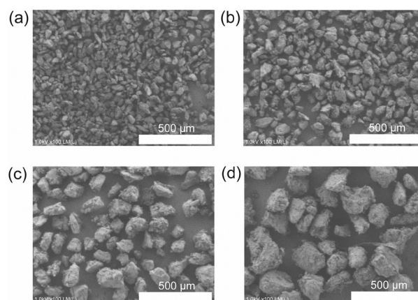
Fig. 6 SEM images of crushed PgFeTPP-DVB10 particles classified using sieves. (a) ~53 \mu\text{m} , (b) 53–100 \mu\text{m} , (c) 100–150 \mu\text{m} , and (d) 150–200 \mu\text{m} .
