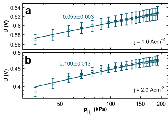
Fig. 3 Logarithmic plot of the voltage at a current density of (a) 1.0 \text{ A cm}^{-2} and (b) 2.0 \text{ A cm}^{-2} against the hydrogen partial pressure. The lines serve as a guide for the eye.
