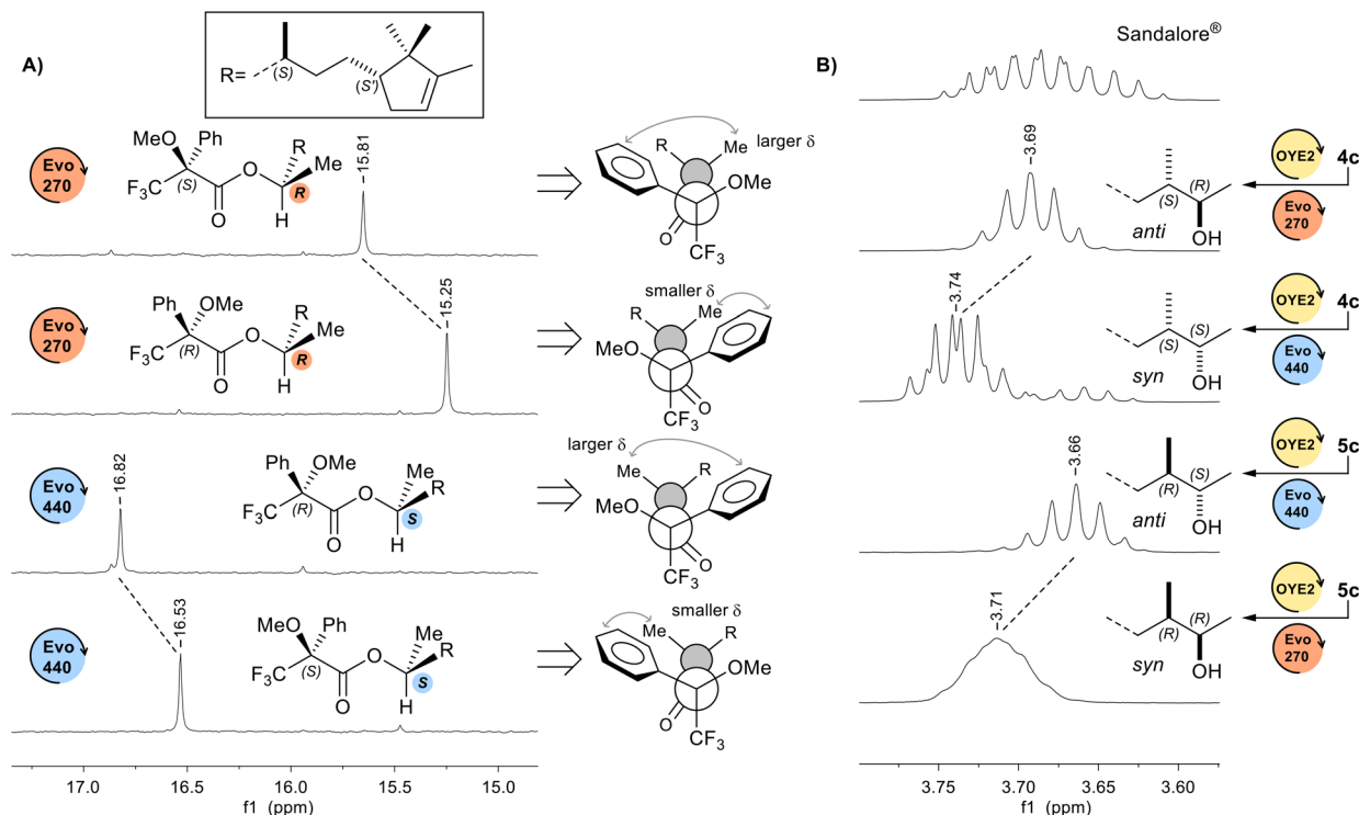
Fig. 3 (A) ^{13}\text{C} -NMR expansion spectra relative to C(1) signal of (R)-MTPA and (S)-MTPA esters of alcohols 1c obtained from the bioreduction of 4c ( \text{CDCl}_3 , 100 MHz). (B) ^1\text{H} -NMR expansion spectra relative to the \text{CHOH} signal of Sandalore® and its diastereoisomers ( \text{CDCl}_3 , 400 MHz).
