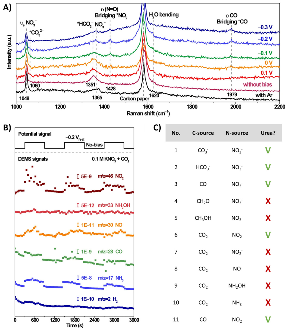
Fig. 16 Mechanistic investigations involving the formation of *O 2 NCO using the CuWO 4 catalyst. (A) In situ Raman spectra at different potentials. (B) Online DEMS at -0.2 V vs. RHE. (C) Control experiment with various C- and N-sources. Adapted from ref. 188 (Open Access).
