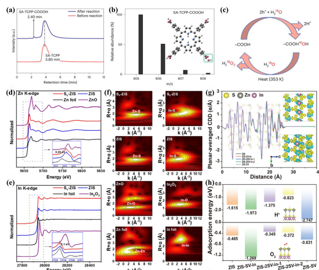
Fig. 6 (a) HPLC for SA-TCPP before and after reaction. 84 (b) The molecular ion peak obtained from the ESI(-)TOF-MS spectrum for the 2.4 min HPLC peak. Inset is the molecular structure of SA-TCPP-COOOH. 84 (c) The mechanism for \text{H}_2\text{O}_2 production on SA-TCPP by holes according to the isotopic experiments. 84 Normalized XANES spectra of S _v -ZIS and ZIS at (d) the Zn K-edge and (e) the In K-edge. The inset is the first derivative of XANES spectra. 86 (f) Wavelet transform analysis of the k^3 -weighted EXAFS for S _v -ZIS and ZIS at the Zn K-edge and the In K-edge. 86 (g) Planar-averaged CDD of ZIS, ZIS-S _v -In, ZIS-2S _v -In, ZIS-2S _v -In-2, and ZIS-S _v . 86 (h) Adsorption energy of H ^+ and O _2 on the S site of the different models. 86
