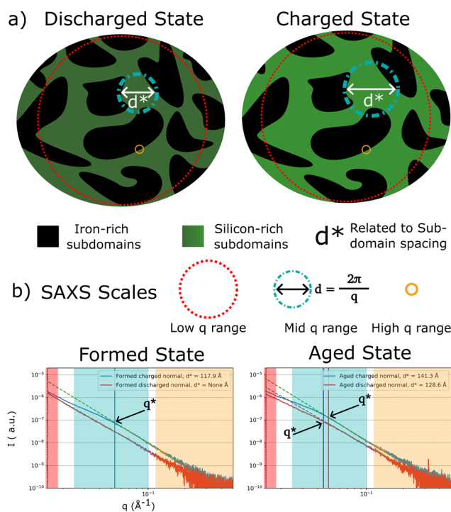
Fig. 4 Concept of SAXS-Analysis of nanostructured material. (a) Shows a stylized depiction of the nanostructure of the Si– \text{FeSi}_2 composite material. (b) Shows two averaged raw SAXS profiles extracted in regular areas for the formed and aged cells respectively, with one curve for the charged state and one curve for the discharged state to highlight the differences in shape caused by the expanding nanostructure.
