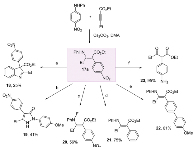
Scheme 4 Enaminoate transformations. a \text{I}_2 , \text{K}_2\text{CO}_3 , DMF, 100 °C, 1 h; b 4-methoxyphenylhydrazine hydrochloride, EtOH, reflux, 16 h; c selectfluor, DCM/ \text{H}_2\text{O} , r.t., 4 days; d \text{Pd}(\text{acac})_2 , Brettphos, \text{K}_3\text{PO}_4 , i PrOH, 1,4-dioxane, 130 °C, overnight; e \text{Pd}(\text{acac})_2 , Brettphos, \text{K}_3\text{PO}_4 , 18-crown-6, (4-methoxyphenyl)boronic acid, 1,4-dioxane, 130 °C, 16 h; f Fe, \text{NH}_4\text{Cl} , EtOH/ \text{H}_2\text{O} , 60 °C, 12 h.
