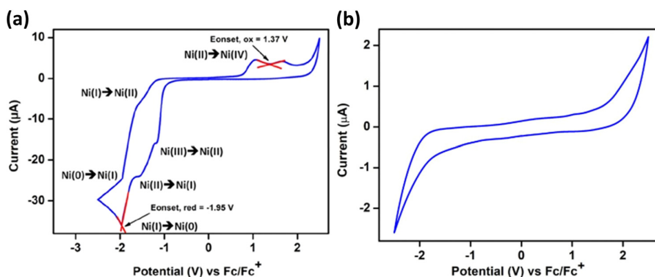
Fig. 14 CV of complex 62 in CH_2Cl_2 (a) and ligand 61 in THF (b), with 0.05 M t -butyl-ammonium-hexafluorophosphate. All potentials were referenced to the Fc/Fc^+ couple. Scan rate = 50 mV s^{-1} . Reproduced from ref. 35 Copyright©2022, American Chemical Society.
