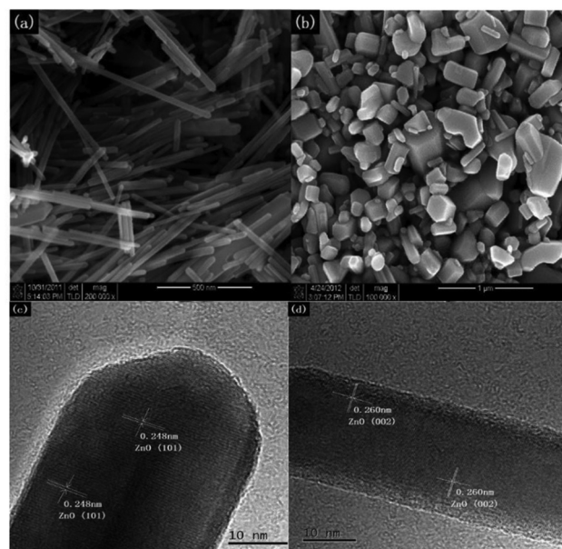
Fig. 13 (Top) SEM imaging of (a) 1D-nanorod \text{ZnO} and (b) bulk \text{ZnO} . (Bottom) TEM imaging of the obtained nanorods. Credit: Z. R. Tang, X. Yin, Y. Zhang and Y. J. Xu, RSC Adv. , 2013, 3 , 5956–5965.
