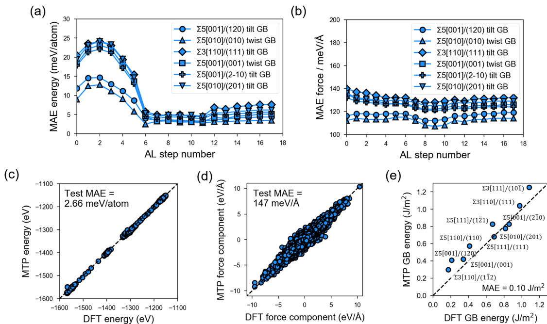
Fig. 3 Test-set accuracy of the trained moment tensor potential (MTP). Mean absolute errors (MAEs) in (a) energies and (b) forces for test \beta -LPS GB structures outside of the active-learning (AL) loop and sampled from 800 K on-the-fly MD runs (6 selected test GB types). Parity plots for MTP vs. DFT (optB88) (c) energies and (d) force components for test GB structures in (a) and (b) that are sampled from 300, 800, and 2000 K MTP-MD runs. (e) Parity plot for MTP vs. DFT GB energy. Dashed line indicates ideal y = x relationship.
