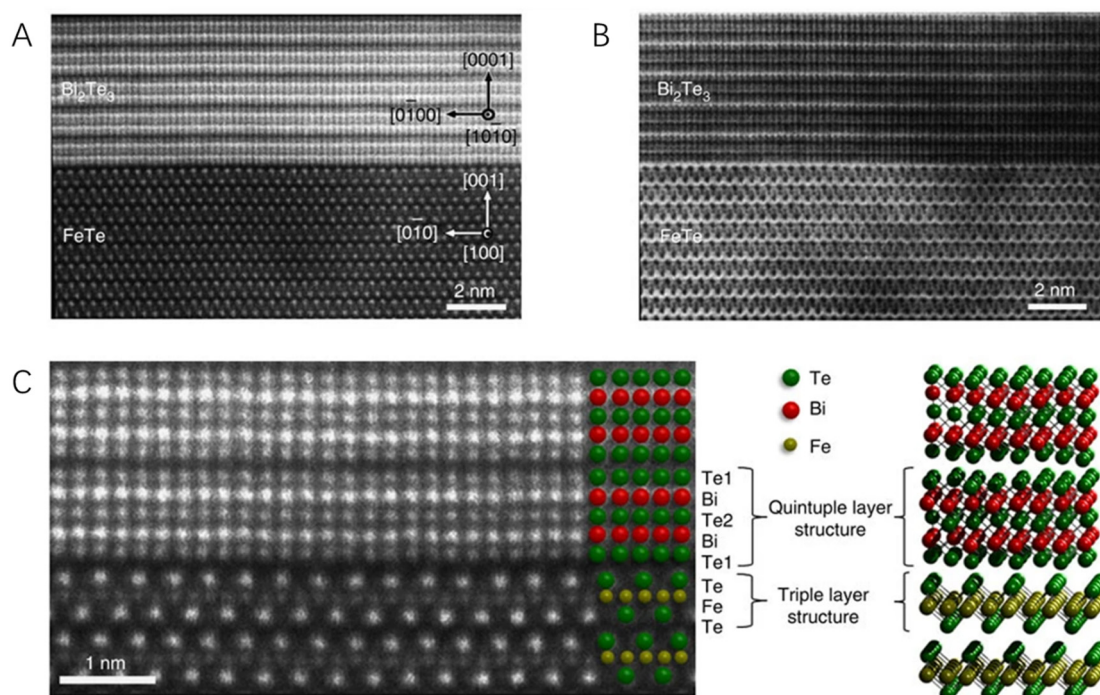
Fig. 5 The scanning transmission electron microscopy micrographs of a \text{Bi}_2\text{Te}_3/\text{FeTe} heterostructure. (A) The HADF image. (B) The annular bright field image. (C) The higher-magnification HADF image showing the atomically sharp interface between \text{Bi}_2\text{Te}_3 and FeTe. Reproduced with permission from ref. 75, copyright Springer Nature.
