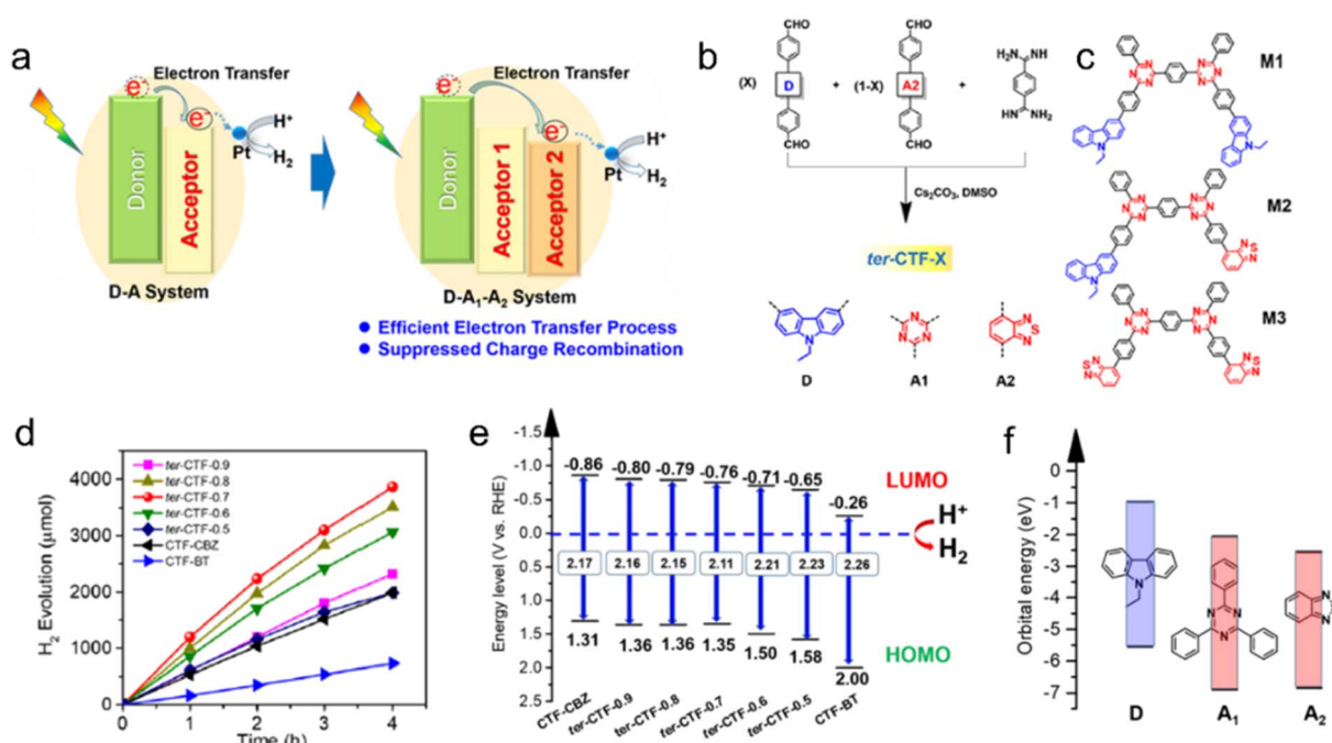
Fig. 9 (a) The photoinduced electron-transfer process of the D–A system and D–A 1 –A 2 system. (b) Rational synthesis of ter-CTF-X (X refers to the percentage of M-CBZ in the total aldehyde monomers). (c) Three proposed model fragments in ter-CTF-X (M1: CBZ combined with triazine; M2: CBZ combined with triazine and BT; and M3: BT combined with triazine). (d) Temporal photocatalytic H 2 evolution over CTFs under visible light by using TEOA as a sacrificial agent. (e) The proposed energy alignments of CTFs based on experimental results. (f) The theoretical energy levels of building blocks. Reproduced with permission from ref. 80. Copyright 2019, American Chemical Society.
