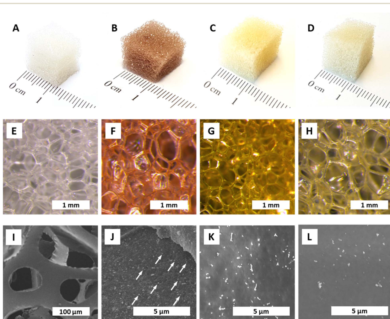
Fig. 1 Aspect and morphology of NPs@PUF. All specimens were synthesized at T_R = 120 \text{ °C} , t_R = 3 \text{ h} , and [M^{*+}] = 0.25 \text{ mM} . Macroscopic aspect (A–D) and optical micrographs (E–H) of pristine PUF and NPs@PUFs: pristine PUF (A and E), AuNP@PUF (B and F); AgNP@PUF (C and G), PdNP@PUF (D,H). SEM micrographs of pristine PUF (I), and NPs@PUFs: AuNP@PUF (J) with some AuNPs indicated with white arrows; AgNP@PUF (K); and PdNP@PUF (L).
