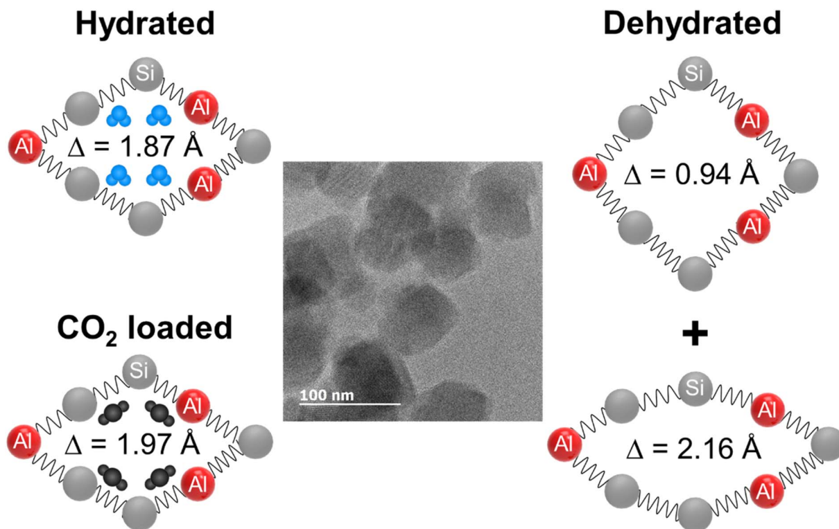
Fig. 5 Schematic illustration of reversible ellipticity of RHO nanosized zeolites upon dehydration and \text{CO}_2 adsorption (adopted with permission from ref. 9, copyright 2020 American Chemical Society).
