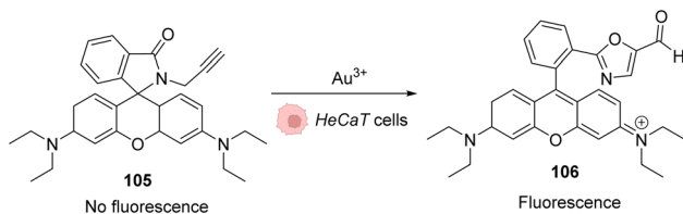
Fig. 35 Generation of fluorescence inside HeCaT cells by the generation of 106 after incubation with \text{Au}^{\text{III}} . 84,85
