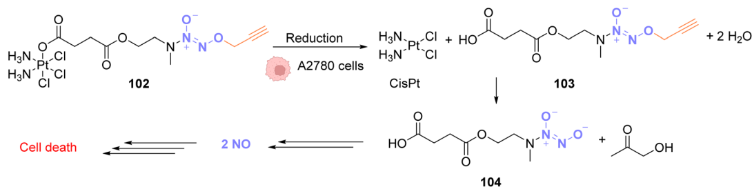
Fig. 34 \text{O}^2 -propargyl cleavage and NO release inside A2780 cells using a platinum(IV) precatalyst of low toxicity. 79
