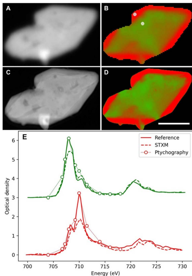
Fig. 13 Comparison between conventional STXM (A and B) and Ptychography (C and D) spectromicroscopy images of \text{Li}_x\text{FePO}_4 micro-platelets. The average optical density (A and C) and the chemical composition map (B and D) where the two chemical components ( \text{LiFePO}_4 and \text{FePO}_4 ) are presented in green and red, respectively (scale bar is 1\ \mu\text{m} ; reconstructed pixel size 5\ \text{nm} ). (E) Point spectra from the dots marked in (B) by conventional STXM (dashed lines) and Ptychographic modes (dotted lines with circles). Reference spectra from pure materials ( \text{LiFePO}_4 , green solid line; \text{FePO}_4 , red solid line) are also shown for comparison. The conventional STXM spectra show distortions that flatten the sharpest peaks, corresponding to energies where the difference in absorption between phases is maximum. The different attenuation overweighs the more abundant phase and instead the Ptychographic spectra more closely match the pure references. Reproduced from ref. 157.
