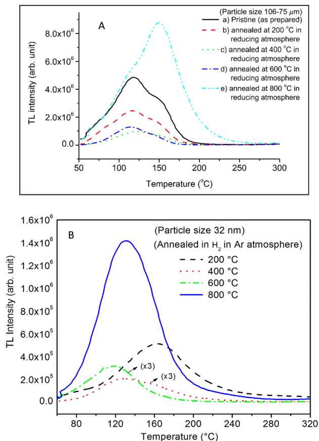
Fig. 15 TL glow curves of SAOE phosphor materials annealed at different temperatures in reducing (10% H 2 in Ar) atmosphere, (A) microcrystalline material (106–75 μm) and (B) nanocrystalline material having particle size \sim 32 nm. Decrease in the TL intensity with particle size without any change in the glow curve structure of the microcrystalline material could be clearly seen in the figure. However, in case of nanomaterial a shift in the peak temperature(s) could also be seen with the annealing temperatures. The TL glow curves of the nanocrystalline material annealed in the temperatures 400 and 600 °C have been multiplied by the factors near these curves and the ordinate (Y-axis) scale needs to be divided these factors to see the actual intensity of these curves.
