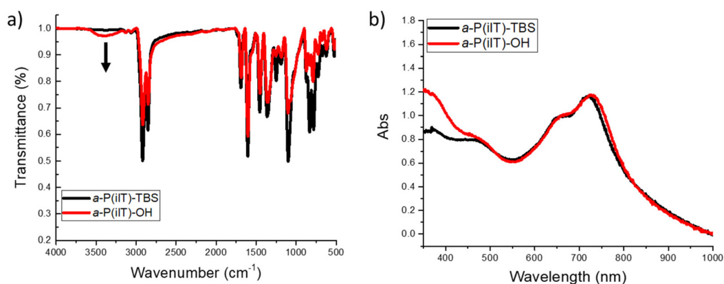
Fig. 1 Fourier-Transform infrared (FTIR) spectra of (a) a\text{-P(iIT)-TBS} and a\text{-P(iIT)-OH} in the solid-state, and (b) UV-vis spectra of a\text{-P(iIT)-TBS} and a\text{-P(iIT)-OH} thin films casted on \text{SiO}_2 .
