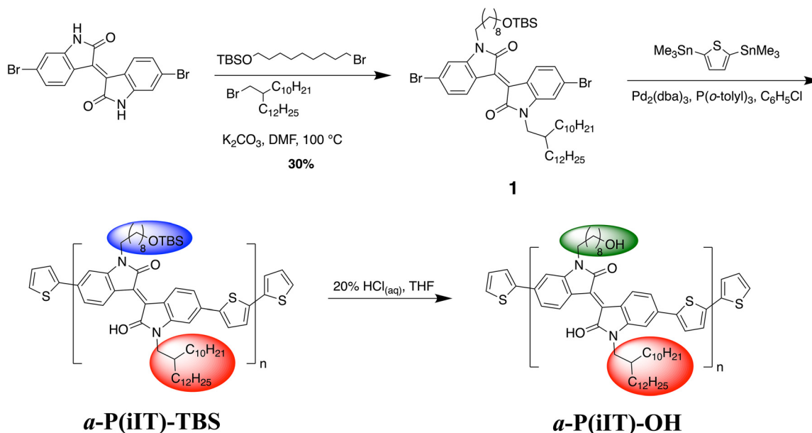
Scheme 1 Synthetic pathway to asymmetric polymer a\text{-P(iIT)-OH} .
