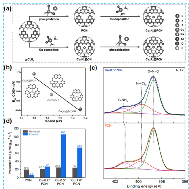
Fig. 20 (a) Scheme of the synthesis of \text{Cu}_1\text{N}_3@PCN and \text{Cu}_1\text{P}_3@PCN . (b) The relationship between the d band center and adsorption energy of \text{COOH}^* on single Cu sites of three model catalysts. 87 (c) N 1s XPS spectra of PCN and Cu-0.5/PCN. (d) Liquid products of methane conversion over PCN and Cu-X/PCN. 88
