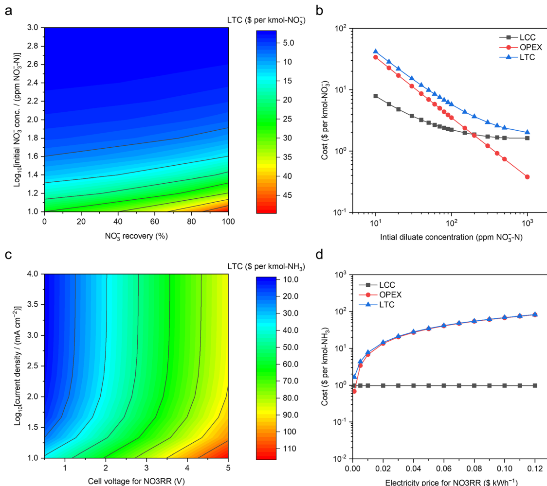
Fig. 5 Techno-economic analysis of upcycling \text{NO}_3^- -N from dilute waste streams. (a) The contour map for the LTC of \text{NO}_3^- concentration by electrodiagnosis with respect to the initial \text{NO}_3^- concentration in the diluate and the designed \text{NO}_3^- recovery from the diluate ( \$0.07 \text{ kW h}^{-1} of electricity cost). (b) LTC, OPEX, and LCC along with the initial diluate concentration ( \$0.07 \text{ kW h}^{-1} of electricity price and 80% of designed \text{NO}_3^- recovery). Based on a typical medium-size commercial electrodiagnosis system (40 cm \times 160 cm for each electrodiagnosis pair, and 250 electrodiagnosis pairs in total), the LCC was calculated via the standard capital recovery method, assuming 40 years of service time, 42 19% as the cost ratio of maintenance to the system, 3% of annual discount rate, 31 83.3% of capacity factor, and 90% of coulombic efficiency. (c) The contour map for the LTC of \text{NH}_3 production by NO3RR in MFAEL with respect to the electrolytic current density and cell voltage ( \$0.07 \text{ kW h}^{-1} of electricity price). (d) The impact of electricity price on the LTC and OPEX of the NO3RR (2.7 V of cell voltage and 250 \text{ mA cm}^{-2} of current density). Capital cost analysis was performed based on a customized medium-size MFAEL reactor with 100 L electrolyte capacity with the total electrode area of 3.36 \text{ m}^2 . The cost of all identified materials and ancillary/auxiliary parts/components was estimated to be \$1164 per system. Considering all unidentified parts (10%) and all other associated costs, 30 the total capital cost of this electrolyzer system was projected to be \$3121 per system. Other assumptions and methodologies are discussed in the ESI†.
