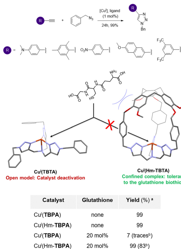
Fig. 10 Typical CuAAC reactions catalysed by \text{Cu}^{\text{I}} ( Hm-TBTA ) with quantitative yields (top). The CuAAC reaction in the presence of the glutathione biothiol: no catalyst inhibition was observed in the case of the caged complex, in contrast to the classical open CuAAC catalyst (bottom). a Catalyst (1 mol%), \text{MeOH}/\text{CH}_2\text{Cl}_2 1:10, 25 °C, and argon atmosphere. b Isolated yields.
